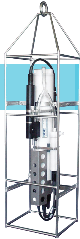
SBE 43 voltage output sensor integrated with SBE 19plus V2 CTD
